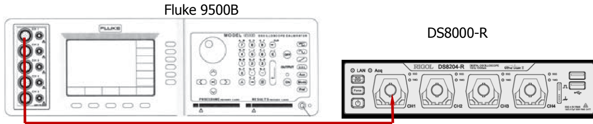
Figure 2-5 Timebase Accuracy Test Connection Diagram
